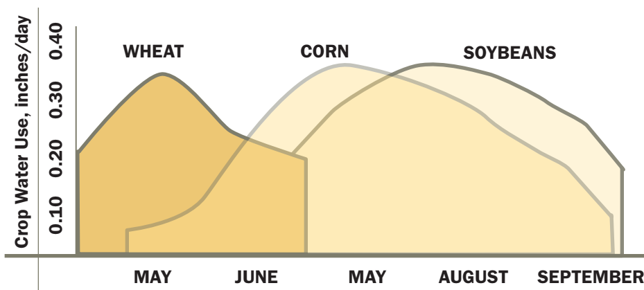
Figure 1. Daily ET during the growing season for wheat, corn and soybean in Colorado. From Broner and Schneekloth, 2003.
