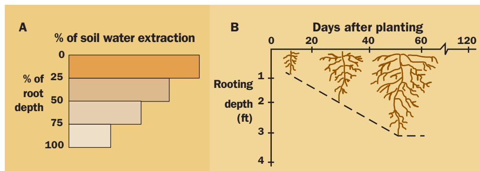
Figure 2. A) Root zone soil water extraction; and B) Plant root development for corn. From Benham (1998).
